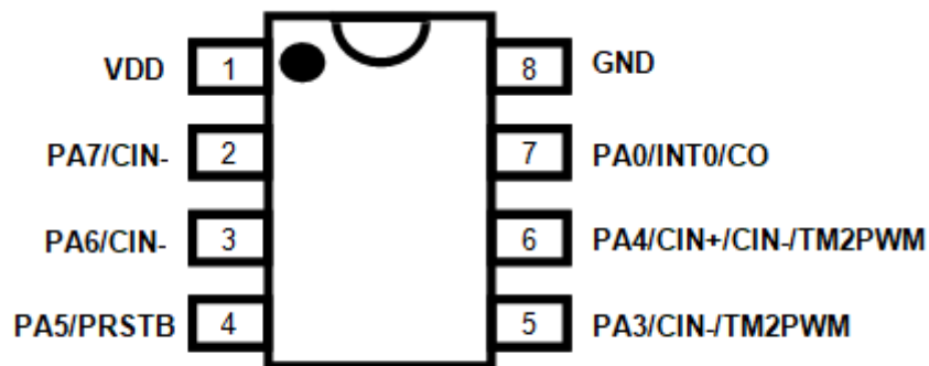
PMS15B/PMS150G -S08 (SOP8-150mil)
