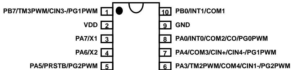
PFS154-M10:MSOP10 (118mil)
