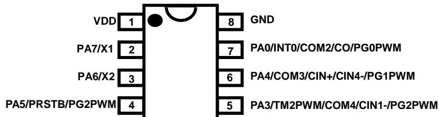
PFS154-S08:SOP8 (150mil)
