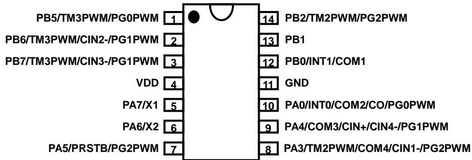
PFS154-S14:SOP14 (150mil)
