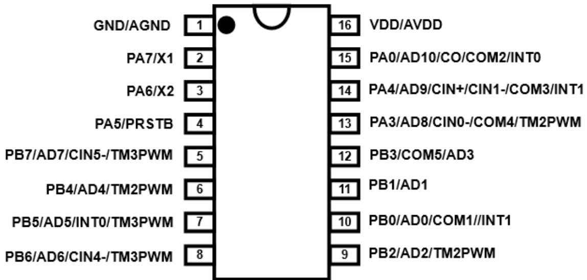
PFS122B-S16B (SOP16B-150mil)
