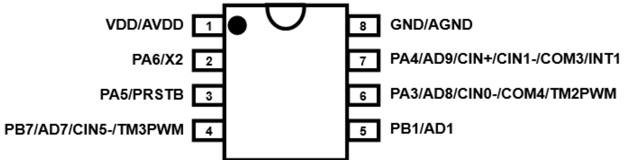
PFS122B-S08 (SOP8-150mil)
