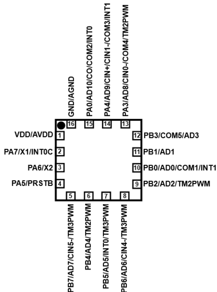
PFS122B-1J16A (QFN3*3-16pin-0.5pitch)
