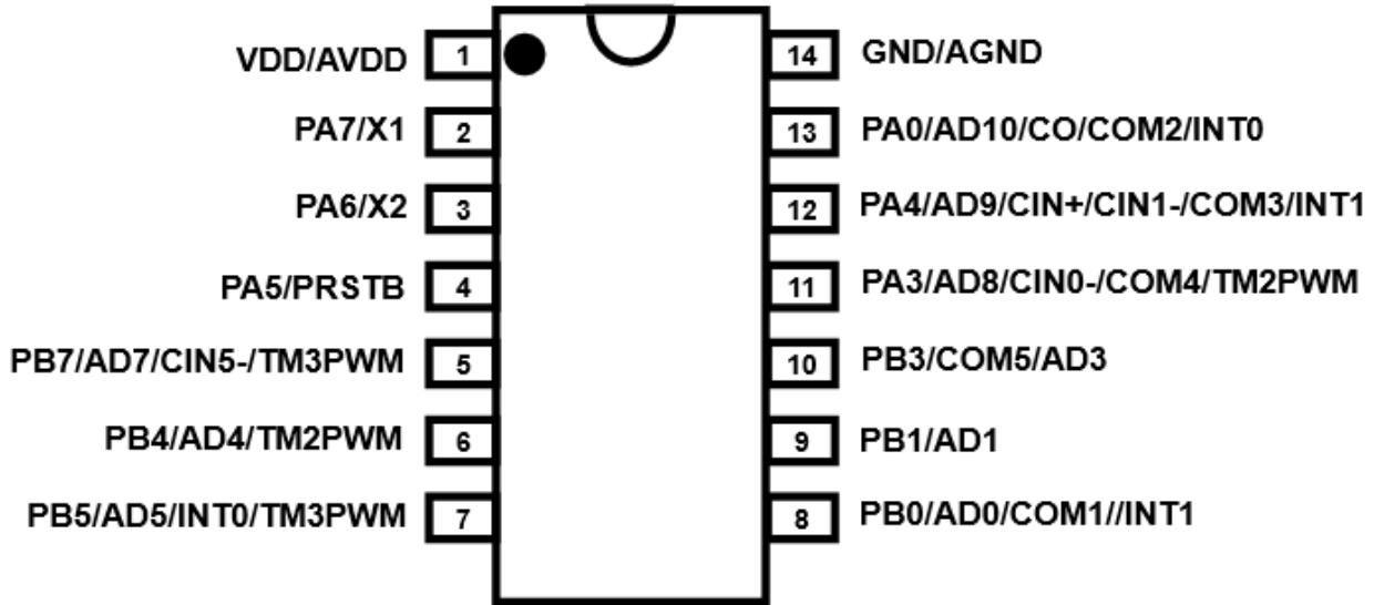
PFS122B-S14 (SOP14-150mil)
