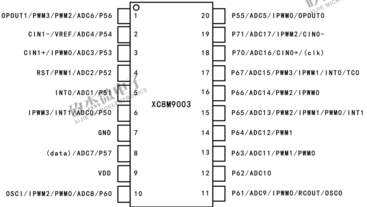
XC8M9003-DIP/SOP20 脚位图
