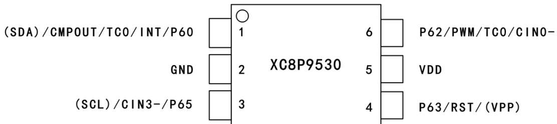
XC8P9530-6PIN 脚位图
